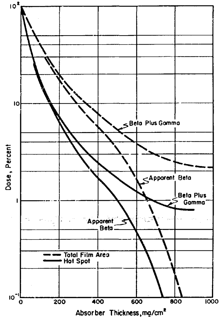
Figure 3.4 Depth-dose measurements on lip tank of B-57B.
